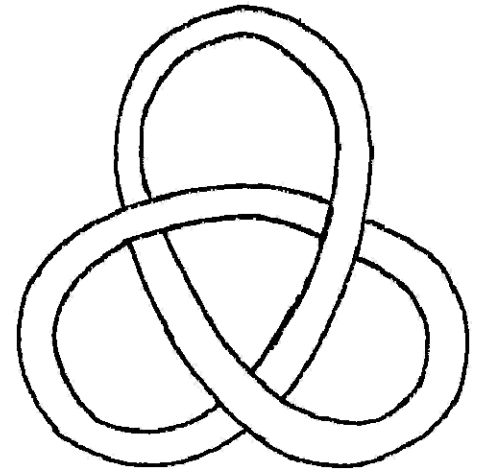
Knot, trefoil
